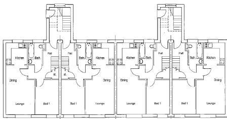
FIRST FLOOR
